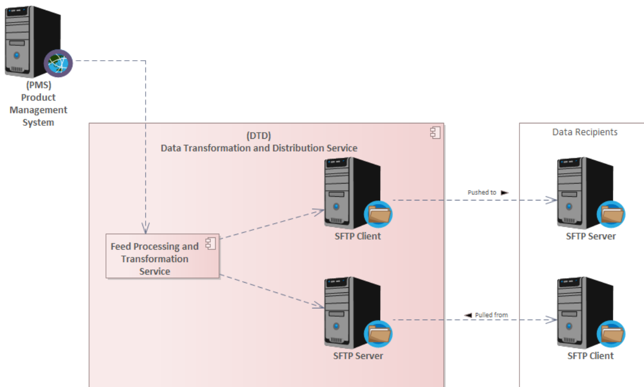
Figure 1 Feed Processing and Transformation Service overview
